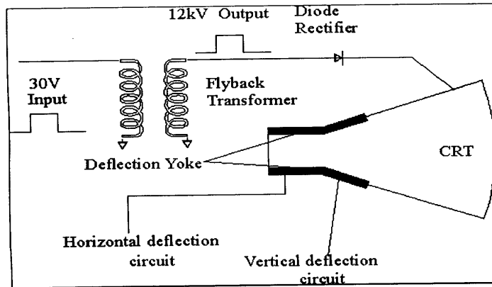
Figure (D) Cross Section of a Typical Video Display Terminal
